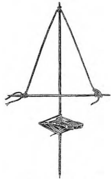
Fig. 139. Drill borer 2622 1 . 52 cm high
