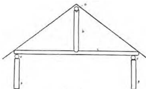
Fig. 149. House construction according to Dr. W. Müller.
